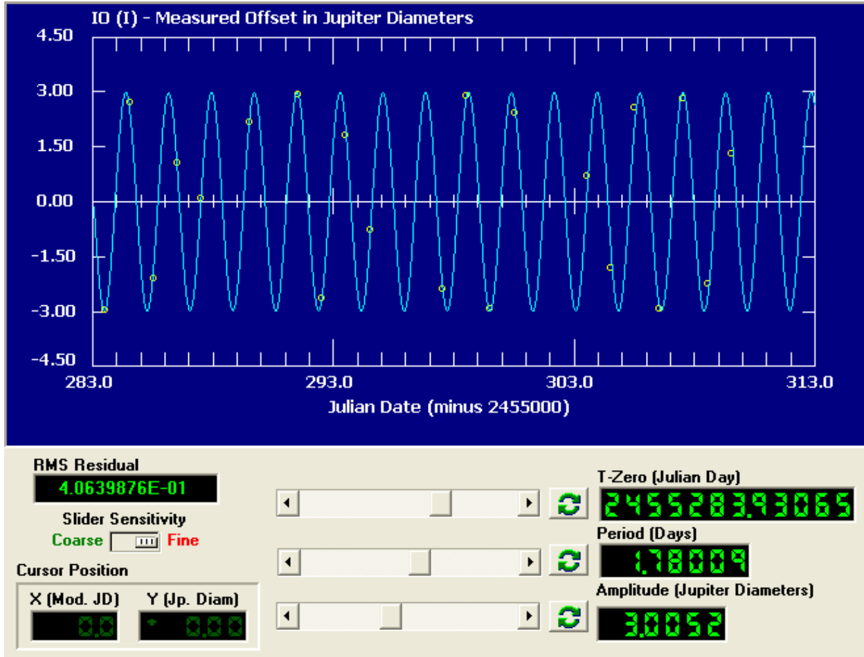
Position vs. time graphs and sine wave fits for moon data
